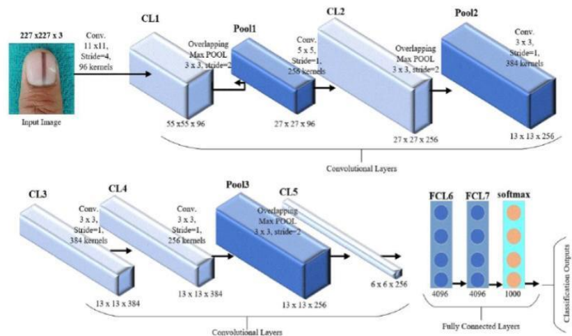
Figure 2: Architecture of CNN
