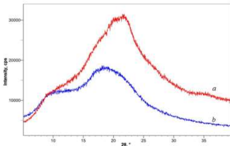
Figure 3. X-ray diffraction patterns of samples: a) CDA treated with KOH; b) CDA initial
