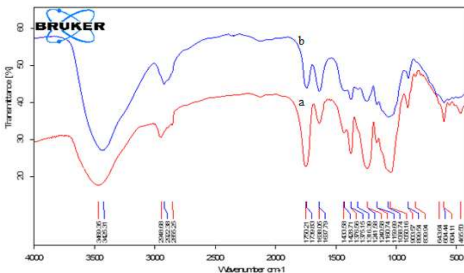
Figure 2. IR spectra of CDA nanofibers (a) and cellulose II nanofibers (b)
