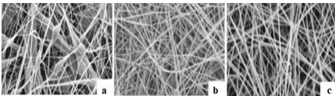
Figure 1. SEM micrographs of nanofibrous nonwoven fabrics obtained from 10% CDA solutions containing 5% (a), 7,5% (b) and 10% (c) water in acetone.
